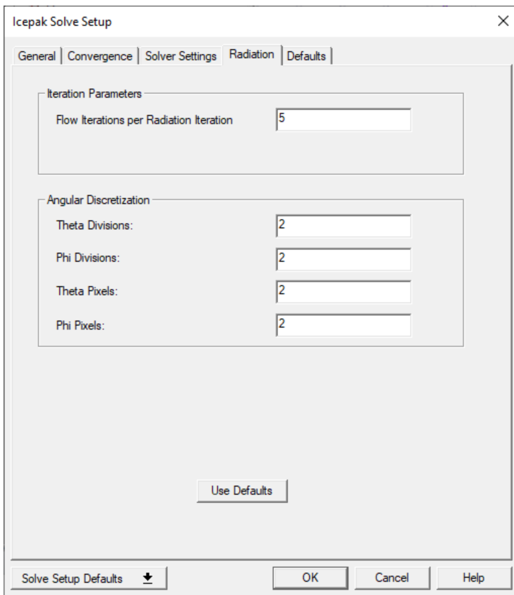
Figure 3-16: Icepak Solve Setup Dialog - Radiation tab
