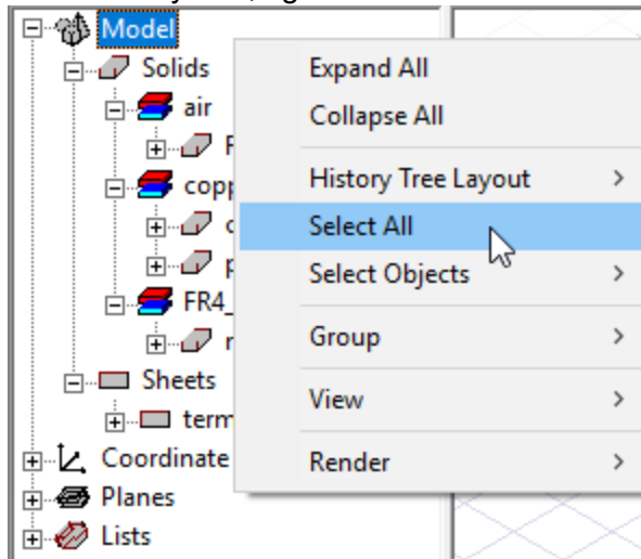
Figure 3-1: History Tree
